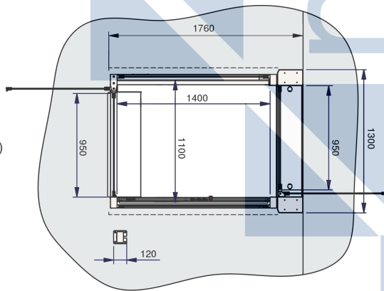
Top floor gate 950 x 1100 mm (Manual opening) (Left)
